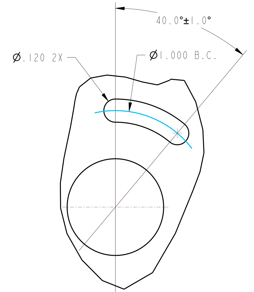
DETAIL B SCALE 4.000 3 EQUAL SPACES
